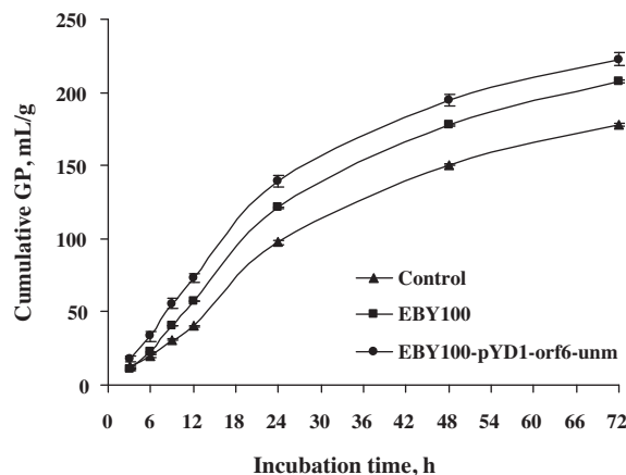
Fig. 4. Cumulative gas production from corn stover by in vitro ruminal cultures. Control, no yeast was added; EB100, the wild type yeast EB100 was added; and EB100-pYD1-orf6-un m , yeast EB100 with surface displayed Orf6-un m was added.
