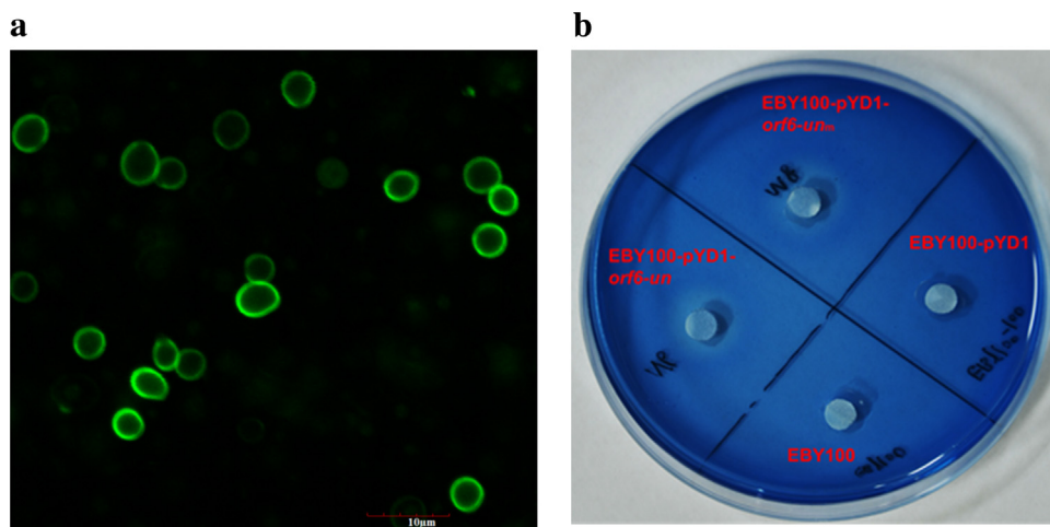
Fig. 1. Immunofluorescence of EB100-pYD1-orf6-unm after staining with anti-V5-FITC antibodies (a) and xylanase activity test of the xylanase displayed on EB100-pYD1-orf6-unm on remazol brilliant blue R-D-xylan agar plate (b).
